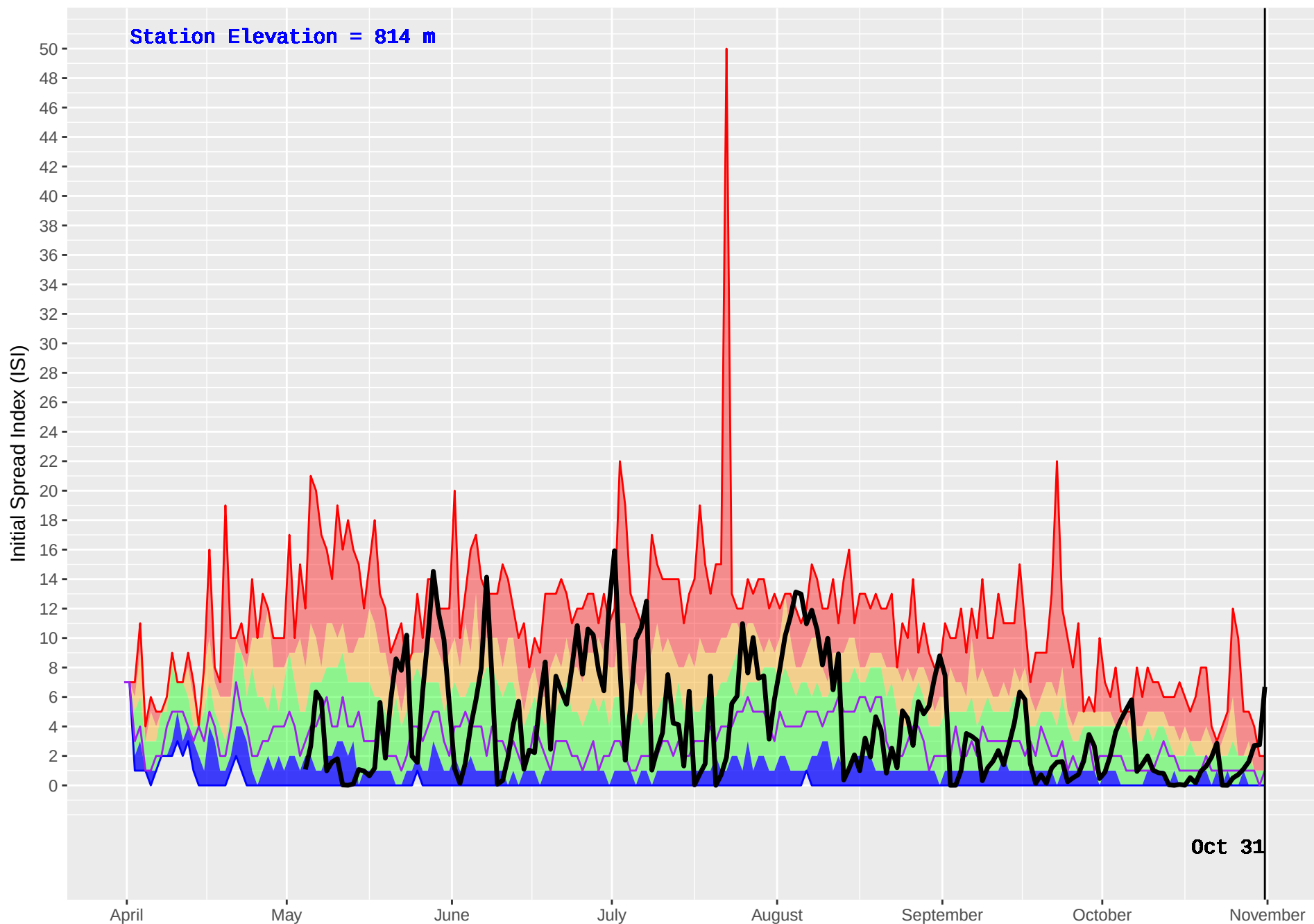
CHILAKO (189) : Historical (1986–2016) and Current (2017) Noon Initial Spread Index (ISI)
