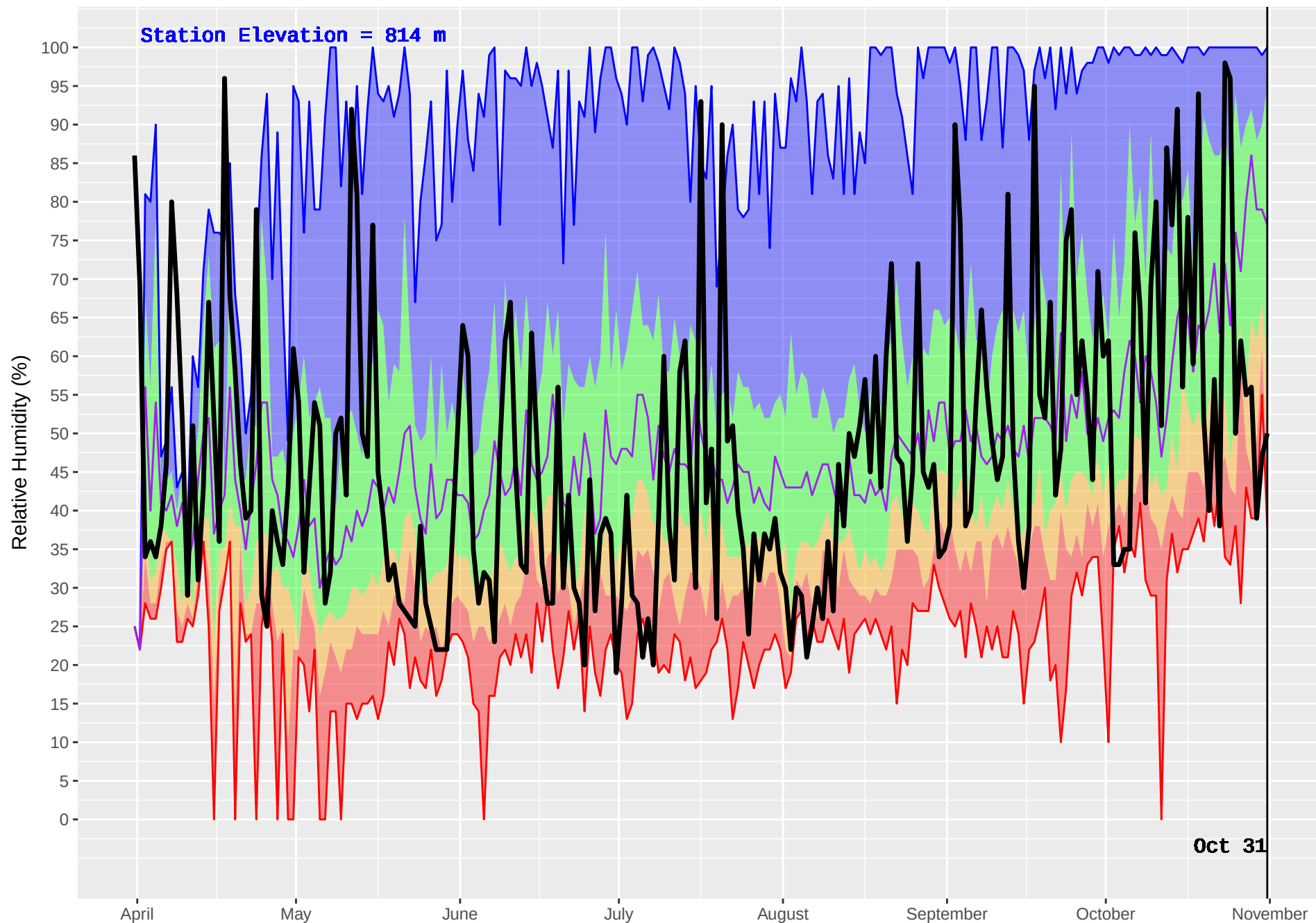
CHILAKO (189) : Historical (1986–2016) and Current (2017) Noon Relative Humidity
