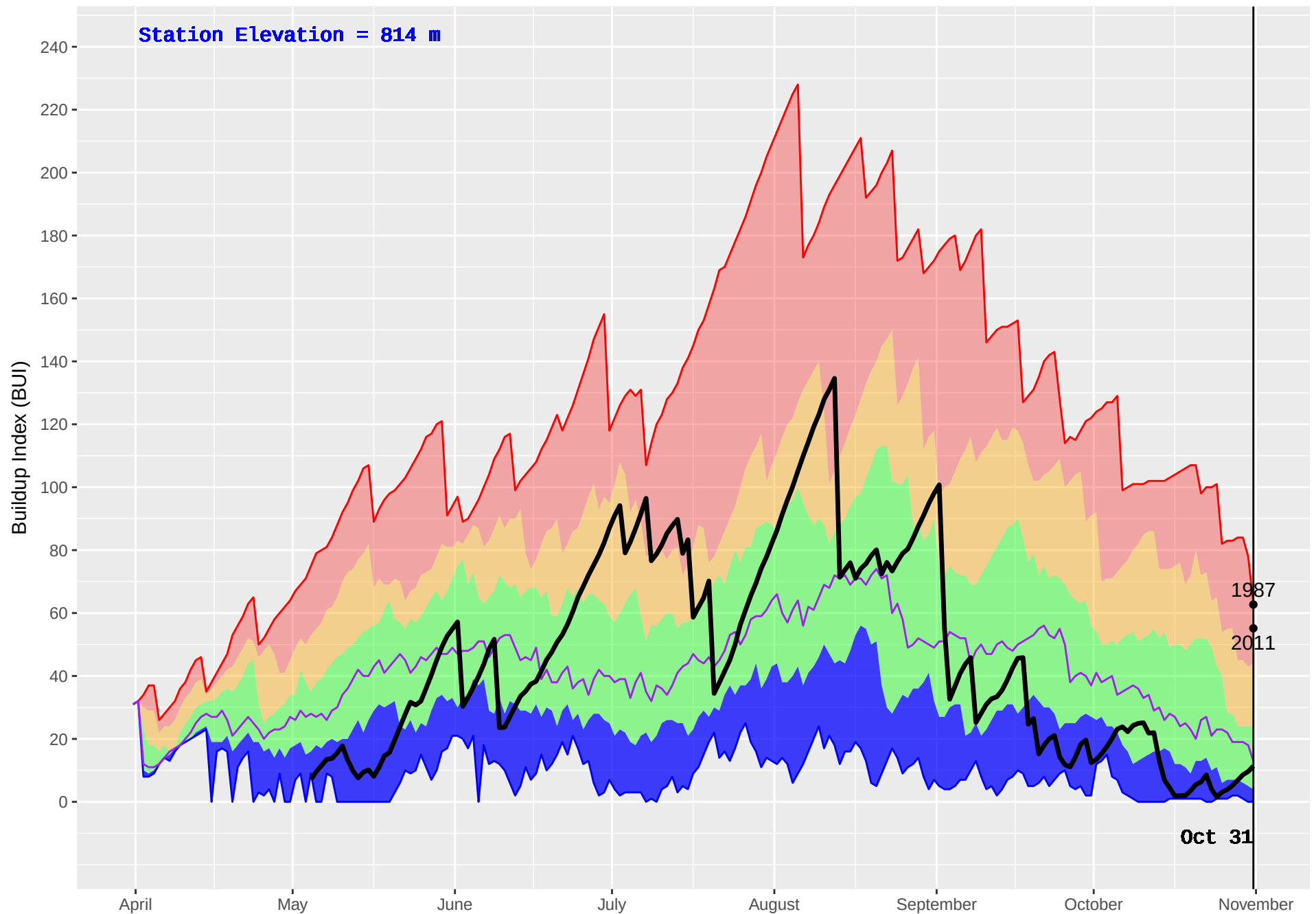
CHILAKO (189) : Historical (1986–2016) and Current (2017) Noon Buildup Index (BUI)
